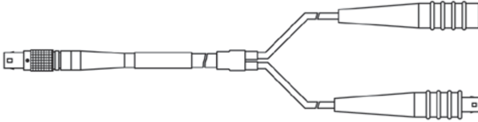
Câble d'interface CAN, OBDII J1962 - Lemo 1B FGC (16mc-8mc), 2m5
