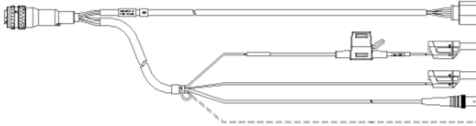
Lambdasondenkabel LSU 4.9, Souriau 8ST12-35 - RB150 (Code 1) - 3.00 m Bananenstecker (22mc-6fc+2mc), 3 9.84 ft CBAL452.1-3 F-00K-106-127 m
