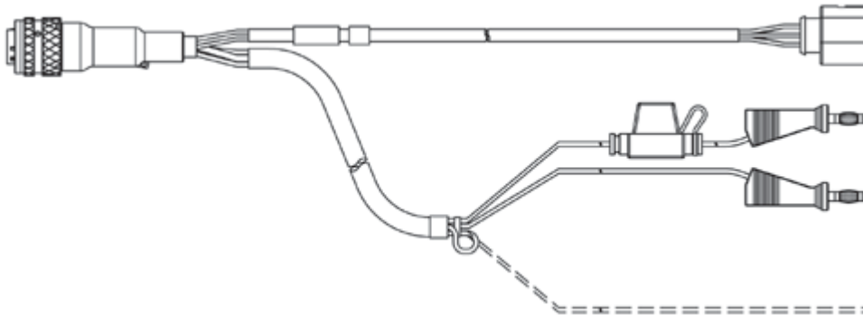
Lambdasondenkabel LSU 4.9, Souriau 8ST12-35 - RB150 (Code 1) - 3.00 m Sicherheitsbananenstecker (22mc- 9.84 ft CBAL4525.1-3 F-00K-110-039 6fc+2mc), 3 m
