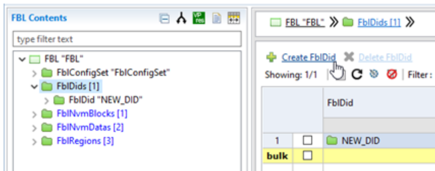
Figure 4.28. ISOLAR GUI for FblDid container with a new DID configured. At the top two buttons allow the user to create or delete an entry
